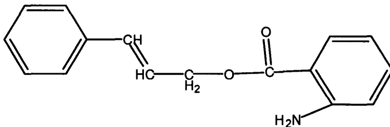
Cinnamyl Anthranilate
